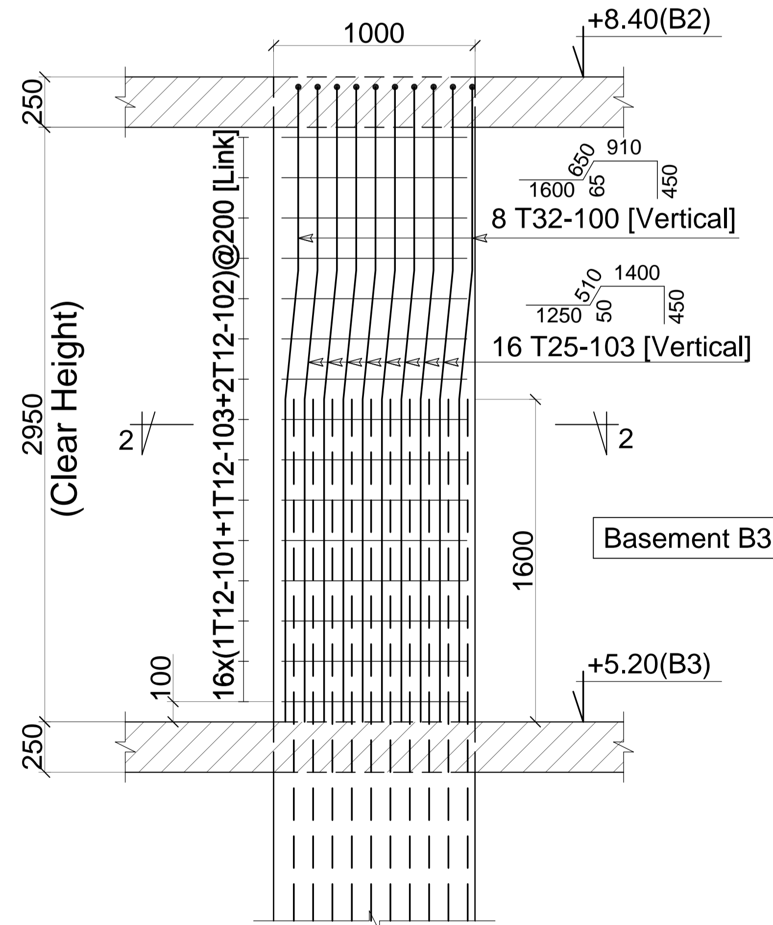
Section 1-1 Scale: 1/50 C1 (3 Nbrs)
