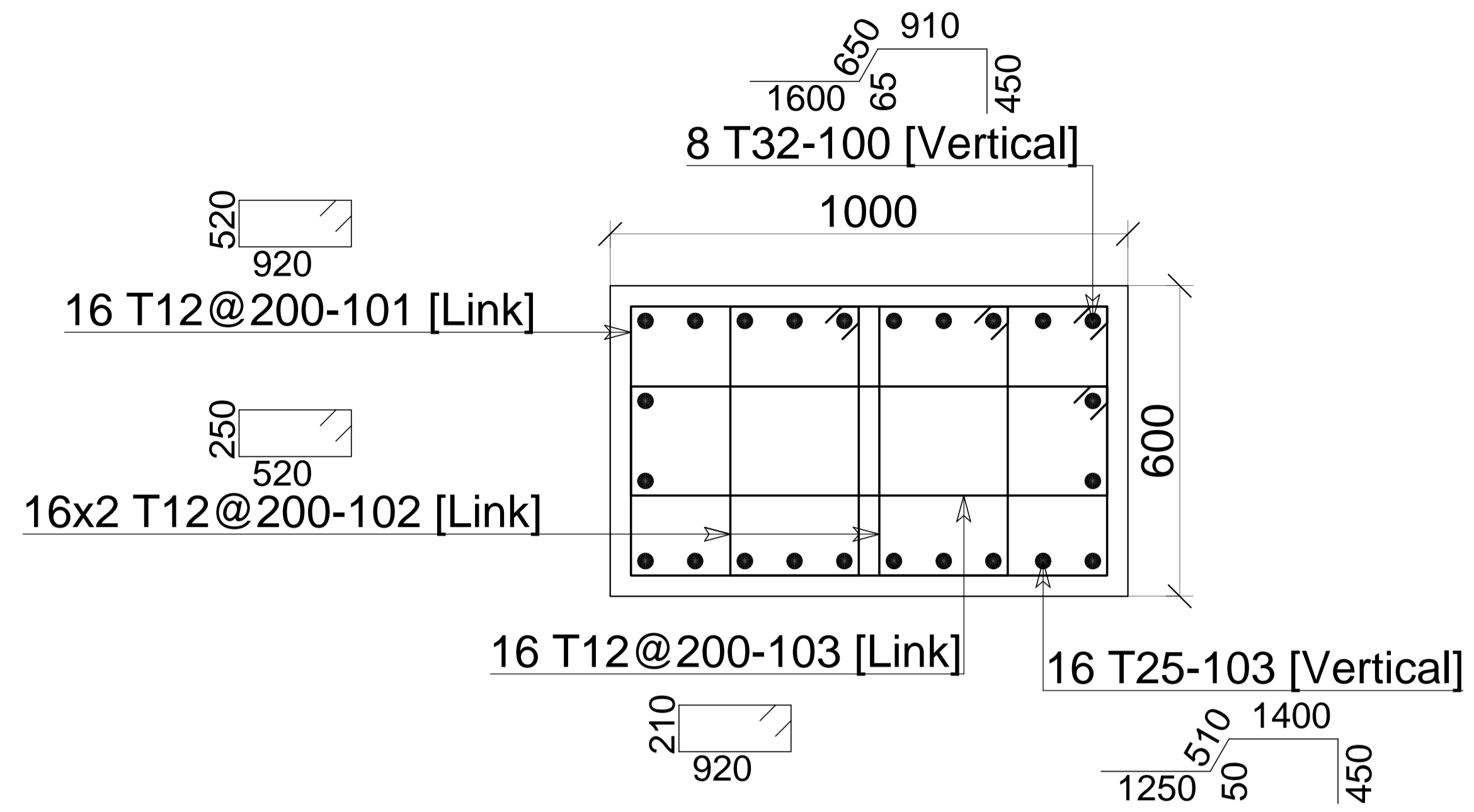
Section 2-2 Scale: 1/25 Column C1 (3 Nbrs)
